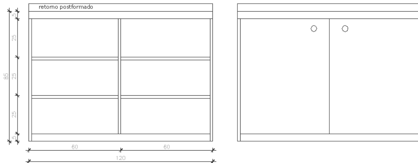
mueble guardavajilla
